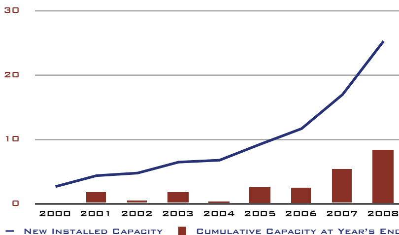
FIGURE 22. UNITED STATES INSTALLED WIND POWER CAPACITY, 2000-2008 (GIGAWATTS CAPACITY)
