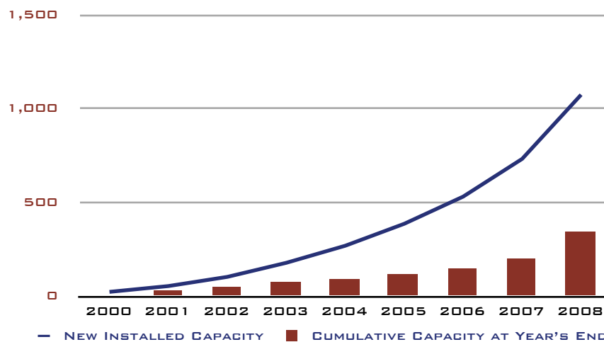
FIGURE 21. UNITED STATES INSTALLED SOLAR POWER CAPACITY, 2000-2008 (MEGAWATTS CAPACITY)
