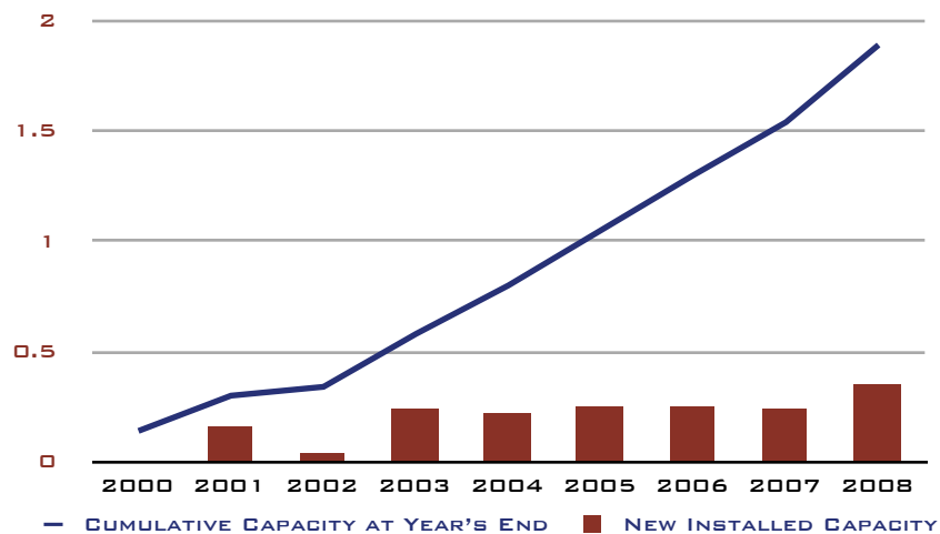
FIGURE 18. JAPANESE INSTALLED WIND POWER CAPACITY, 2000-2008 (GIGAWATTS CAPACITY)
