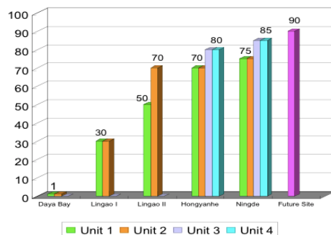
FIGURE 13. PROGRESSIVE LOCALIZATION OF CPR-1000 (PERCENT OF REACTOR COMPONENTS MANUFACTURED IN CHINA)
