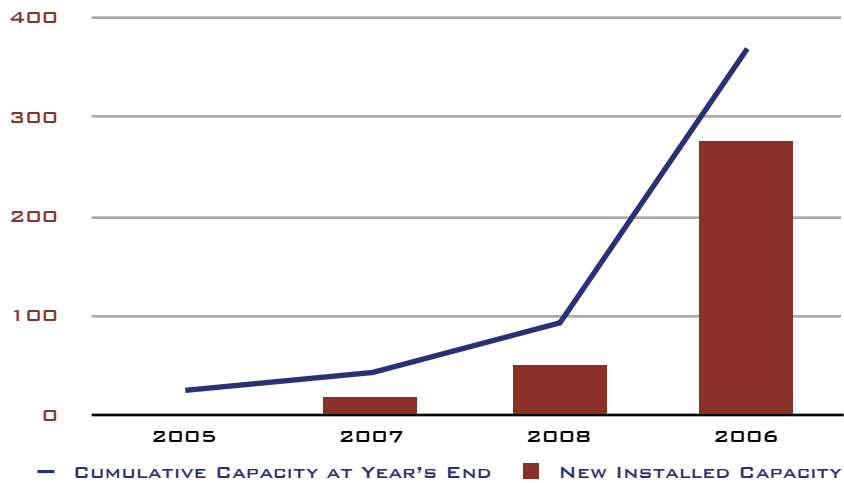
FIGURE 19. SOUTH KOREAN INSTALLED SOLAR POWER CAPACITY, 2005-2008 (MEGAWATTS CAPACITY)
