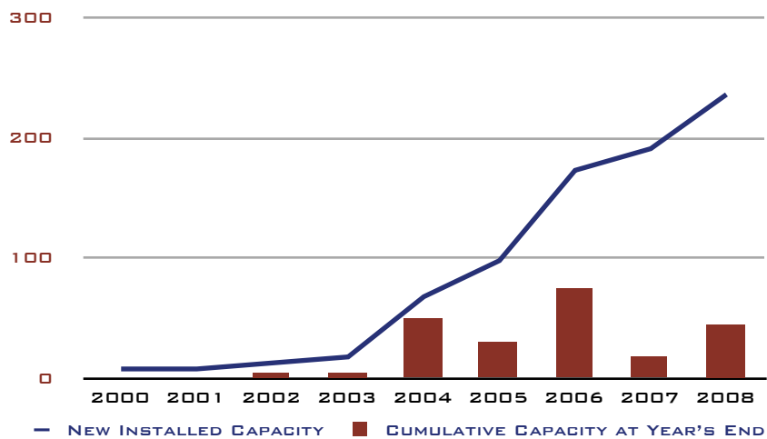
FIGURE 20. SOUTH KOREAN INSTALLED WIND POWER CAPACITY, 2000-2008 (MEGAWATTS CAPACITY)
