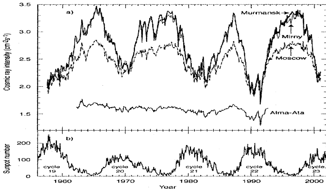
Figure 2-9: Solar Modulation of Galactic Cosmic Rays, 1957-2001
