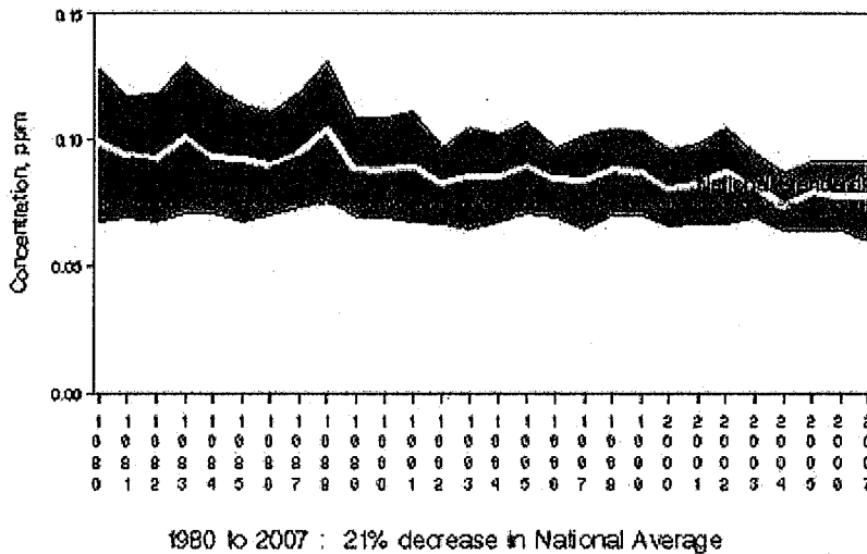
Ozone Air Quality, 1980 — 2007 (Based on Annual 4th Maximum 8-Hour Average) National Trend based on 269 Sites
