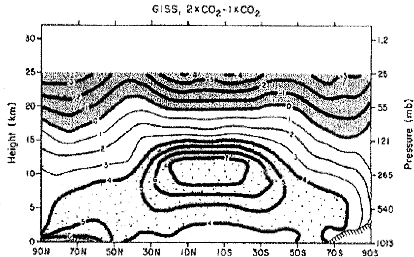
Figure 10. North-South vertical-cross section showing Hansen's early GCM's model change in temperature (oC) that would accompany a doubling of atmospheric CO 2 . There is no way a doubling of CO 2 and an extra 3.7 W/m 2 blockage of OLR to space could lead to such extreme upper tropospheric temperature rises. These large temperature increases occurred because of Hansen's unrealistic upper level water vapor assumptions.
