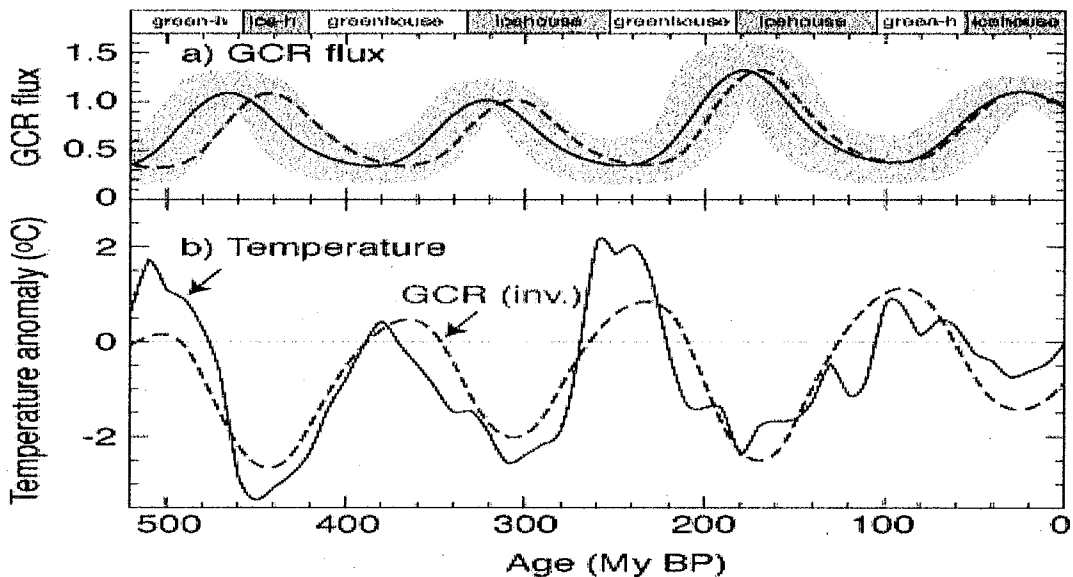
Figure 2-10: Galactic Cosmic Rays and Climate: Past 500 myr
