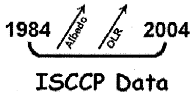
Figure 1. Data sources utilized in this study. NCEP/NCAR Reanalysis data (1950-2008) of wind, thermodynamics and OLR derived radiation, and data from the International Satellite Cloud Climatology Project (ISCCP) for the period of 1984-2004 which contain a variety of radiation components are examined.
