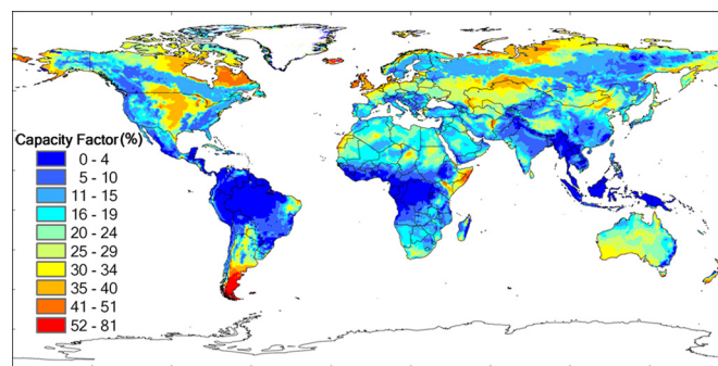
Fig. 7. Global distribution of onshore capacity factor (%) for winds at 100 m with exclusion of permanent snow/ice-covered areas such as Antarctic and Greenland.
