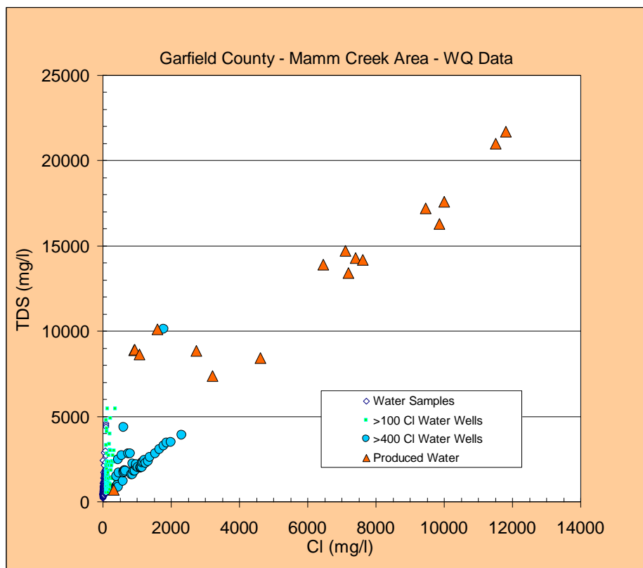
Figure 13. Plot of 704 surface and ground water samples from the Mamm Creek study area for chloride versus TDS.
