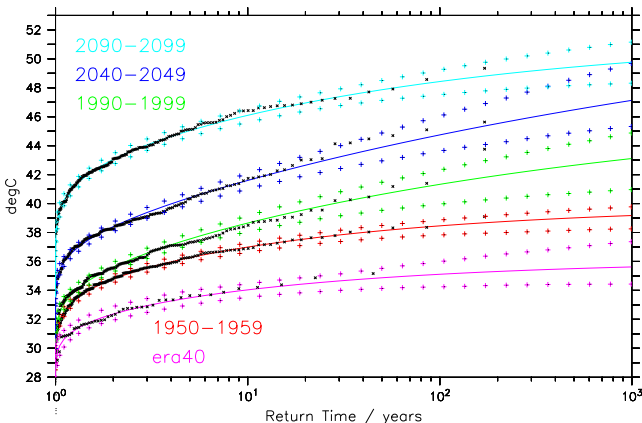
Figure 1. GEV-fit for annual-maximum T_{2m} at a location in Southern France ( 2^{\circ} E, 42^{\circ} N ) as a function of return time (see (2)) for different time slices, together with the values derived from ERA-40 for the period 1958-2002. The colored crosses give the 95%-confidence interval, based on a bootstrap with 1,000 repetitions, and the black symbols are the simulated annual-maximum values.
