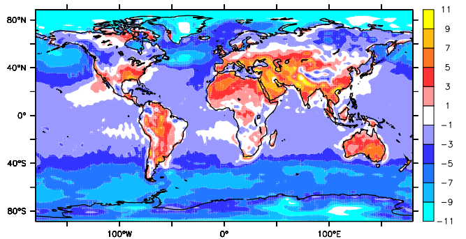
Figure 2. Differences of T_{100} between Essence and ERA-40 for the entire ERA-40 period (1958-2100).
