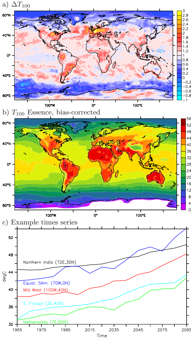
Figure 3. (a) Difference between 2090-2099 and 1990-1999 of T_{100} , expressed as a multiple of the ensemble mean temperature change during the same period. Red (blue) colors mean that T_{100} grows faster (slower) than the mean temperature. (b) T_{100} from Essence for the period 2090-2100, corrected for the bias with respect to ERA-40 (see Fig. 2). (c) Time series of T_{100} at selected places, bias corrected using ERA-40. The years denote the middle of the respective time-slice of ten years.
