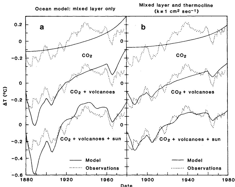
Fig. 5. Global temperature trend obtained from climate model with sensitivity 2.8^\circ\text{C} for doubled \text{CO}_2 . The results in (a) are based on a 100-m mixed-layer ocean for heat capacity; those in (b) include diffusion of heat into the thermocline to 1000 m. The forcings by \text{CO}_2 , volcanoes, and the sun are based on Broecker (25), Lamb (27), and Hoyt (48). Mean \Delta T is zero for observations and model.
