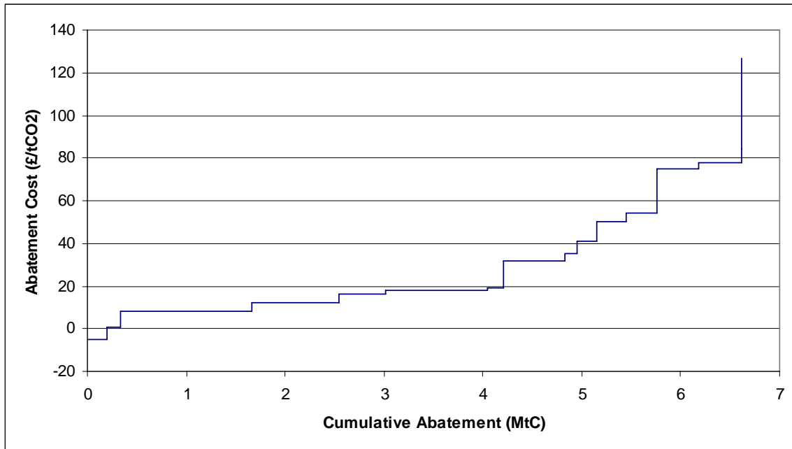
Figure 6 Illustrative CO 2 cost vs abatement curve for CO 2 avoided by the deployment of biomass heat.
