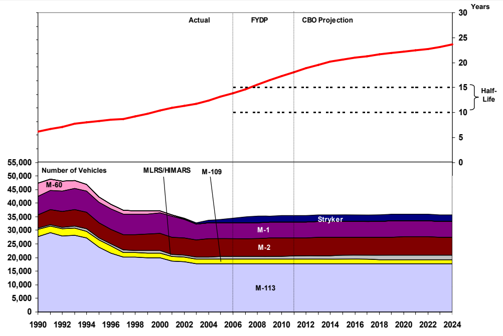
Age and Inventory of Army Ground Combat Vehicles Under CBO's Evolutionary Alternative
